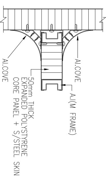
DETAIL G SCALE 1:3
