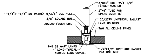
3 AD2000 GRID SUPPORT DETAIL W/A
