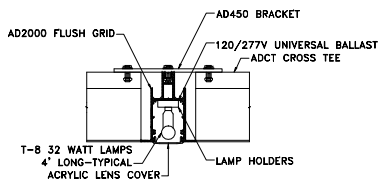
4 AD2000 GRID DETAIL W/A
