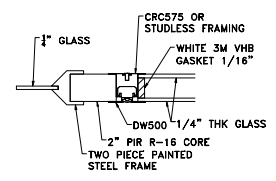
7 SINGLE & FLUSH WINDOW DETAIL W/A
