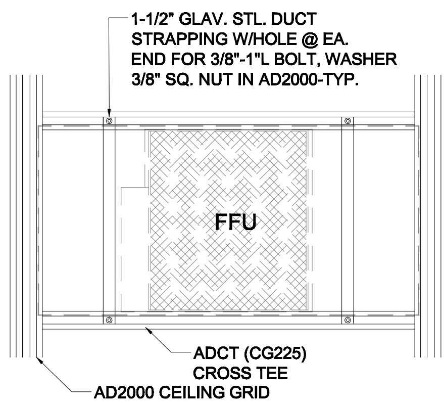
1 FFU SEISMIC ATTACHMENT DETAIL N/A
