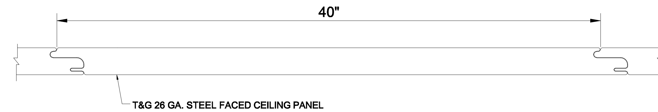
3 WALL & CEILING PANEL SECTION N/A
