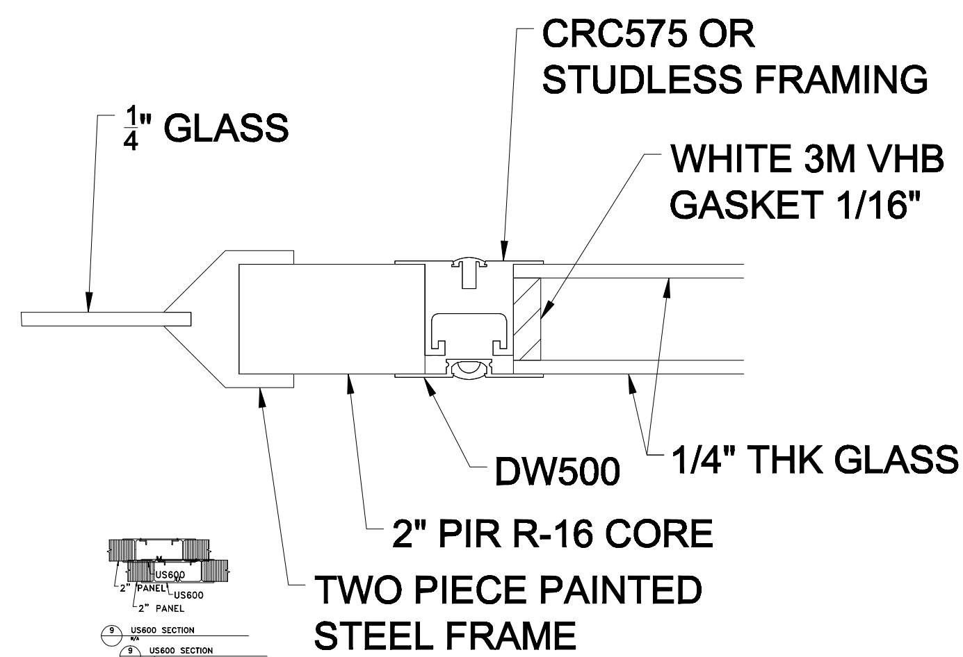
8 SINGLE & FLUSH WINDOW DETAIL N/A
