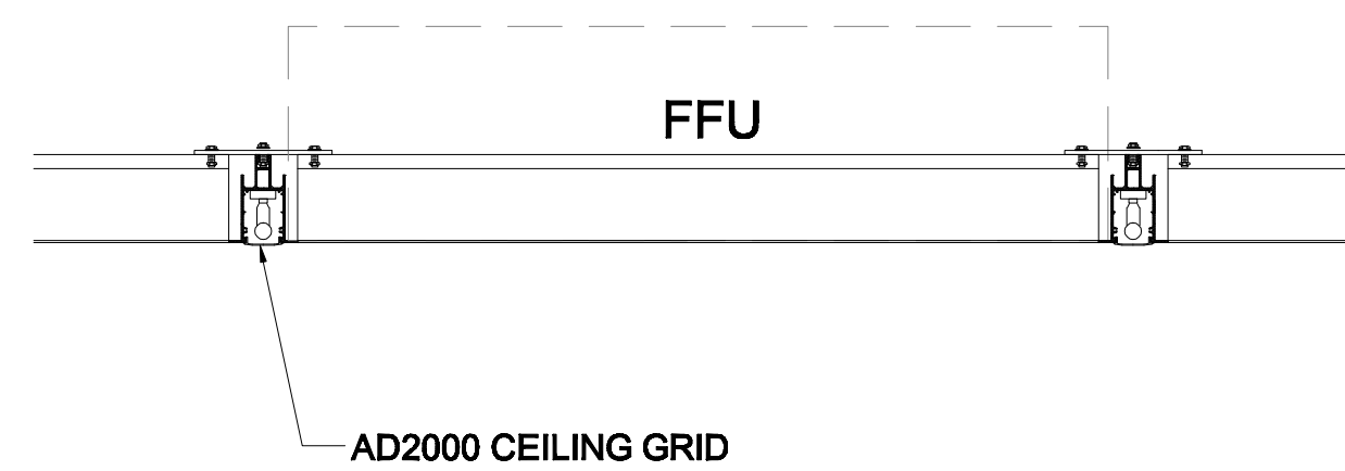
2 PARTIAL CEILING SYSTEM SECTION N/A
