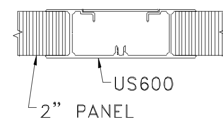
5 AD2000 GRID DETAIL N/A
